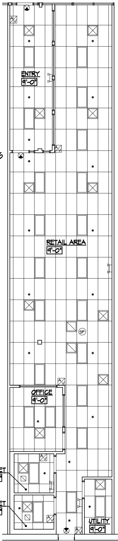
CEILING PLAN SCALE: 3/32" = 1'-0"
