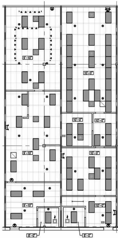
CEILING PLAN SCALE: 3/32" = 1'-0"
