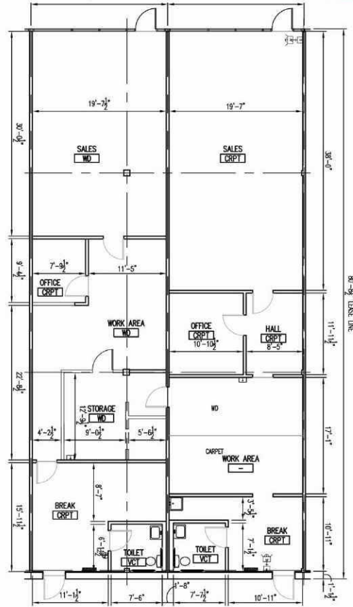
FLOOR PLAN SCALE: 3/32" = 1'-0"
