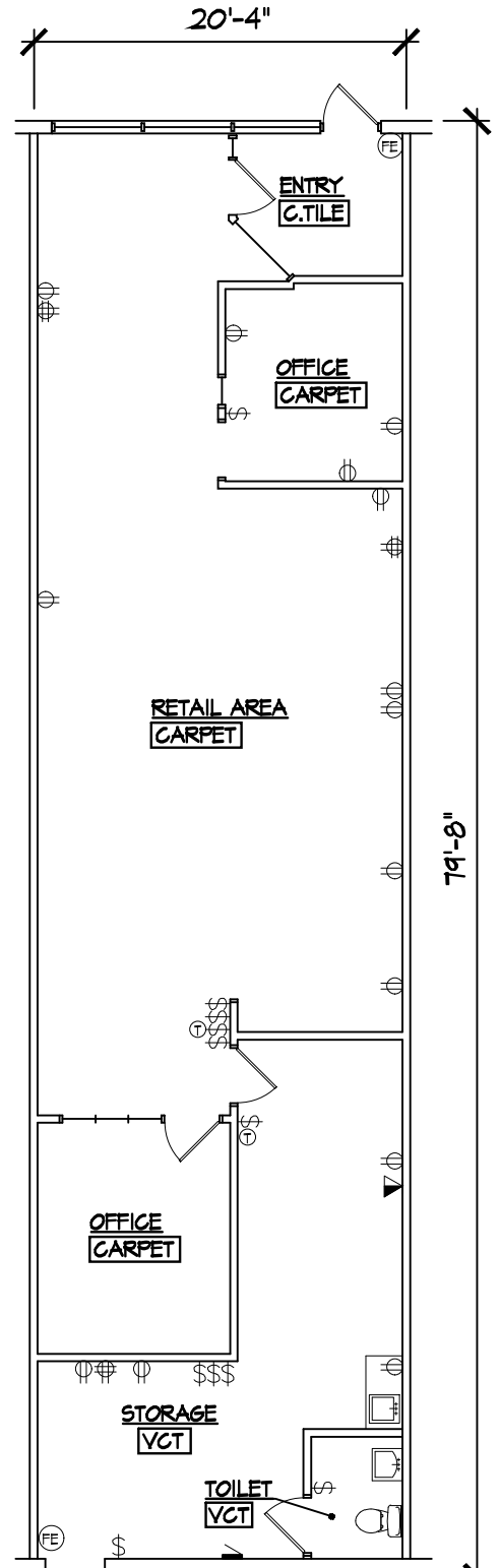
FLOOR PLAN
