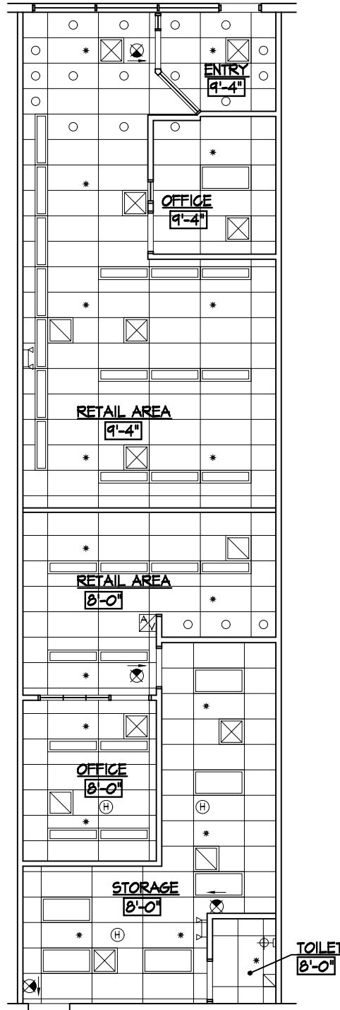
CEILING PLAN
