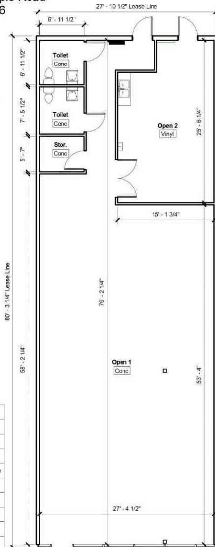
1 Floor Plan 3/32" = 1'-0"
