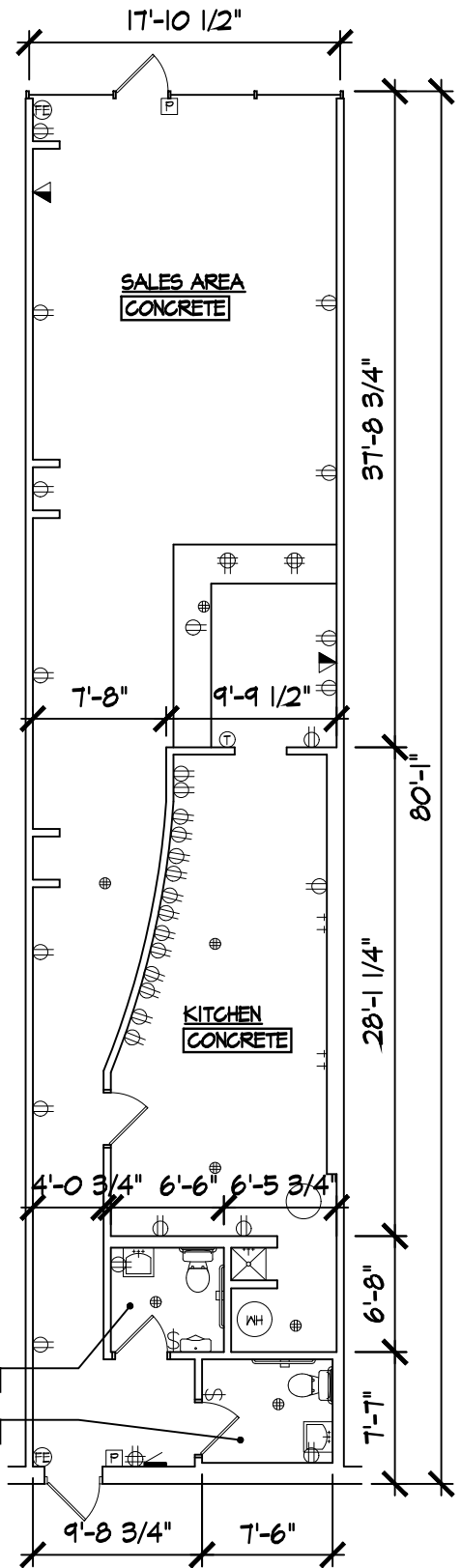
FLOOR PLAN SCALE: 3/32" = 1'-0"
